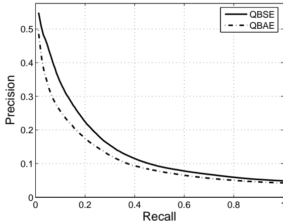
Fig. 1. Precision-Recall curves for query-by-semantic-example (QBSE) and query-by-acoustic-example (QBAE).
